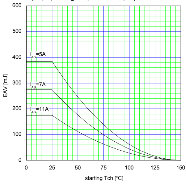
Maximum Avalanche Energy vs. starting Tch E(AV)=f(\text{starting Tch}):V_{CC}=60V, I(AV)\leq 11A
