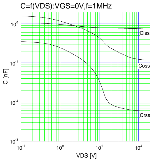
Typical Capacitance
