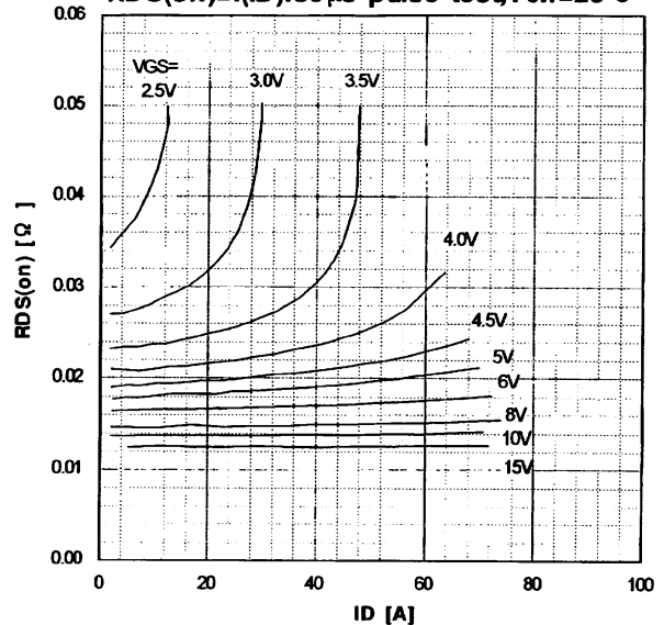
Typical Drain-Source on-state Resistance vs. ID R DS(on) =f(ID):80 μs pulse test,T ch =25°C
