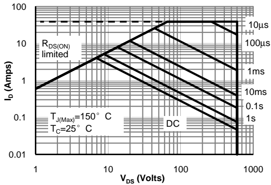
Figure 9: Maximum Forward Biased Safe Operating Area for AOWF11N60 (Note F)
