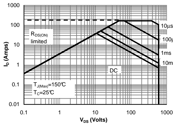
Figure 11: Maximum Forward Biased Safe Operating Area for AOT42S60 (Note F)
