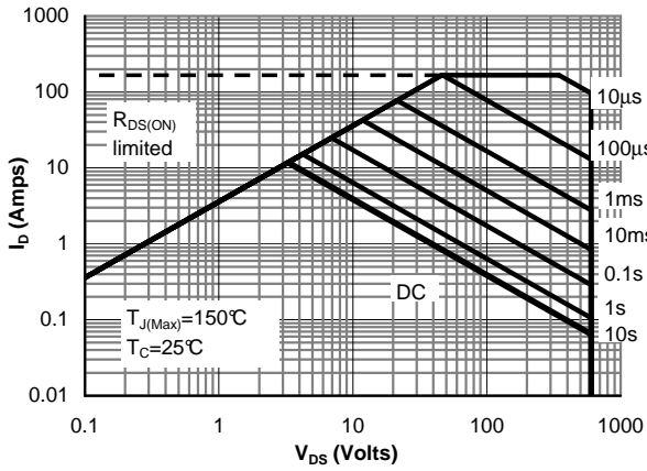
Figure 13: Maximum Forward Biased Safe Operating Area for AOTF42S60L(Note F)
