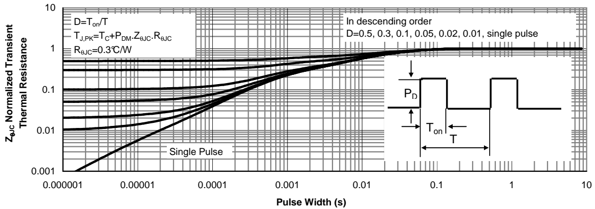
Figure 16: Normalized Maximum Transient Thermal Impedance for AOTF42S60(Note F)
