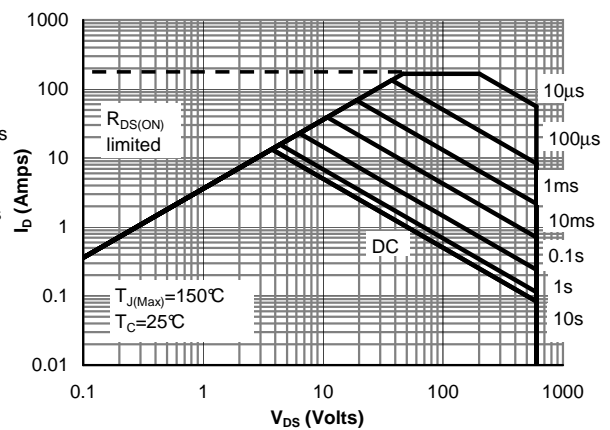
Figure 12: Maximum Forward Biased Safe Operating Area for AOTF42S60 (Note F)
