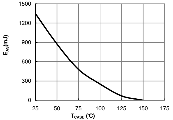
Figure 14: Avalanche energy
