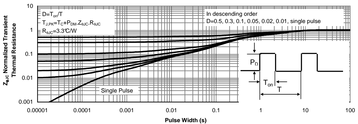
Figure 18: Normalized Maximum Transient Thermal Impedance for AOTF42S60L (Note F)
