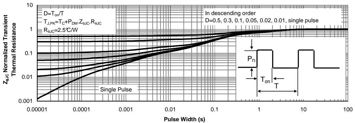
Figure 17: Normalized Maximum Transient Thermal Impedance for AOTF42S60(Note F)
