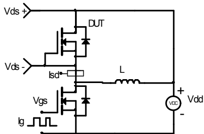
Diode Recovery Test Circuit & Waveforms
