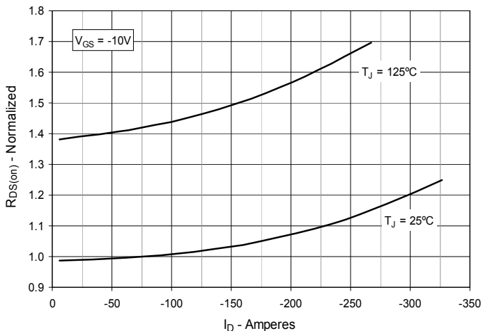
Fig. 5. R_{DS(on)} Normalized to I_D = -70\text{A} vs. Drain Current
