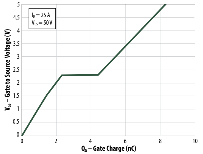
Figure 6: Gate Charge
