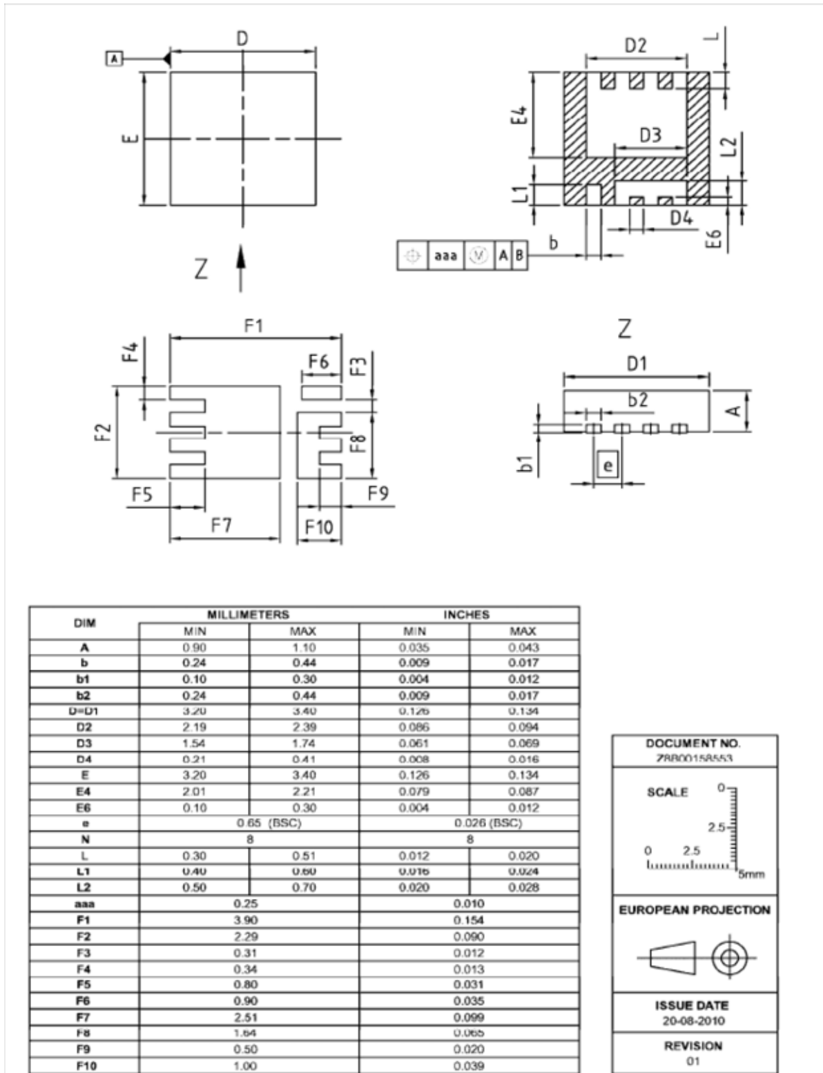
Figure 1 Outlines PG-TSDSON-8 ( fused leads ), dimensions in mm/inches
