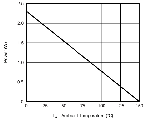
Power, Junction-to-Ambient
