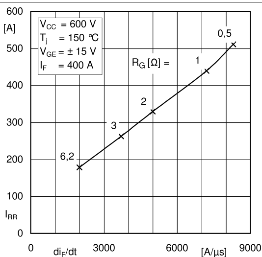
Fig. 11: CAL diode peak reverse recovery current
