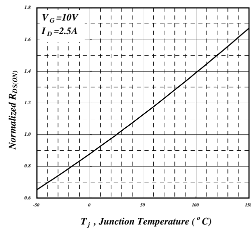
Fig 4. Normalized On-Resistance
