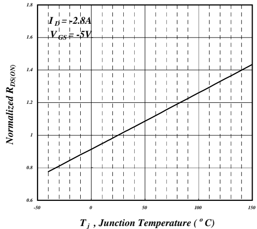
Fig 4. Normalized On-Resistance
