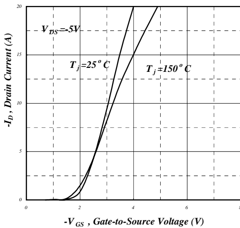
Fig 11. Transfer Characteristics
