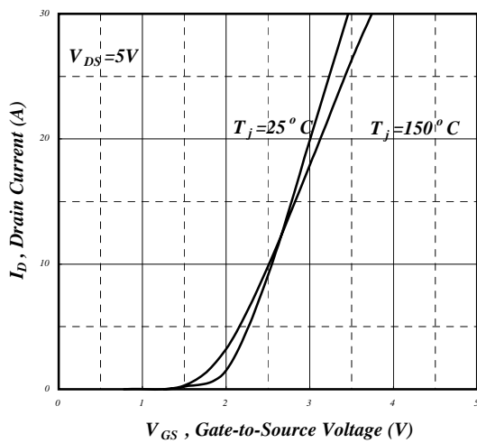
Fig 11. Transfer Characteristics
