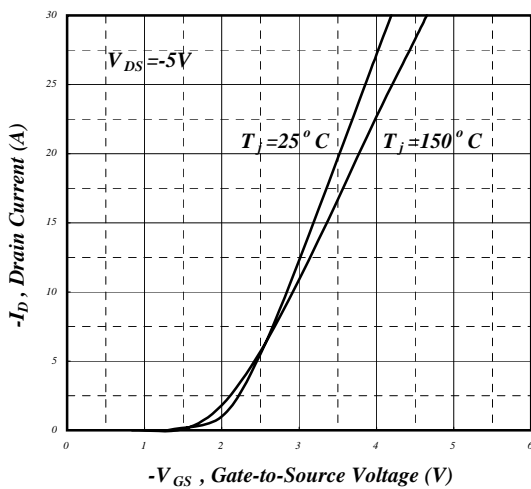
Fig 11. Transfer Characteristics
