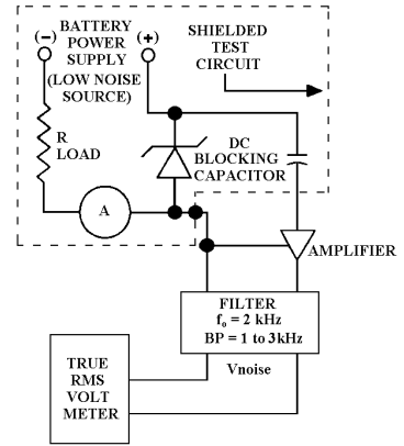
NOISE TEST CIRCUIT FIGURE 2
