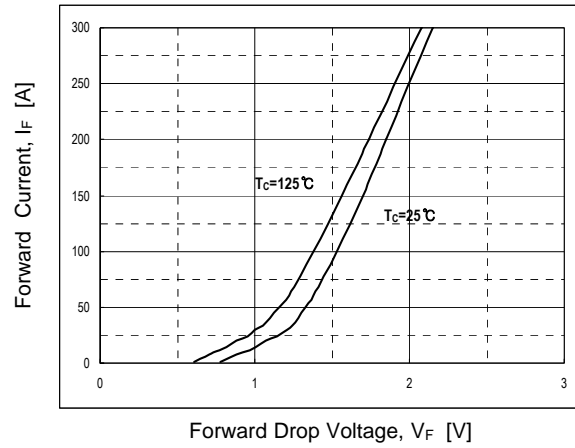
Fig 14. Forward characteristics
