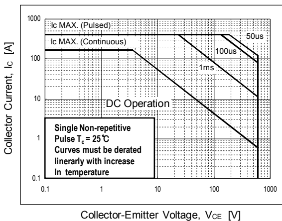
Fig 11. SOA characteristics
