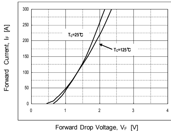
Fig 14. Forward characteristics
