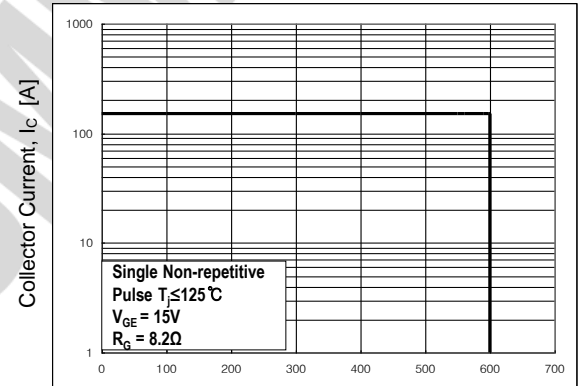
Fig 10. RBSOA Characteristic
