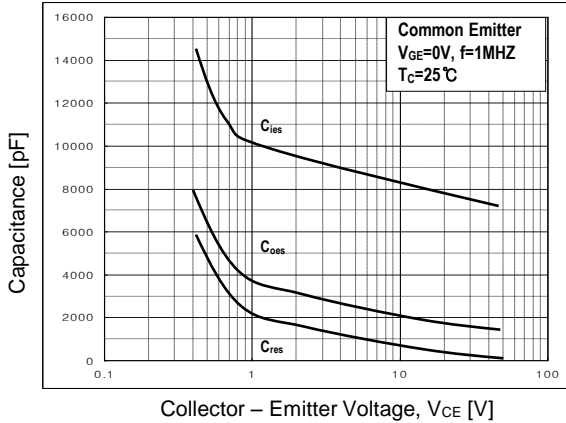
Fig 7. Capacitance characteristics
