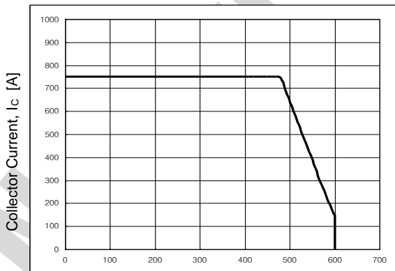
Fig 11. SCSOA Characteristic
