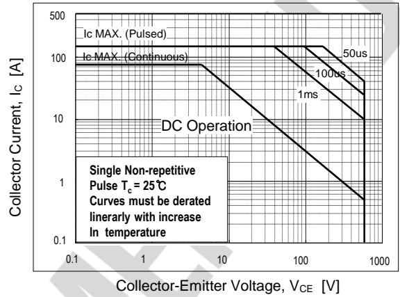
Fig14. SOA characteristics
