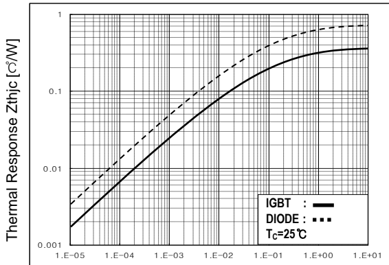
Fig 9. Transient Thermal Impedance
