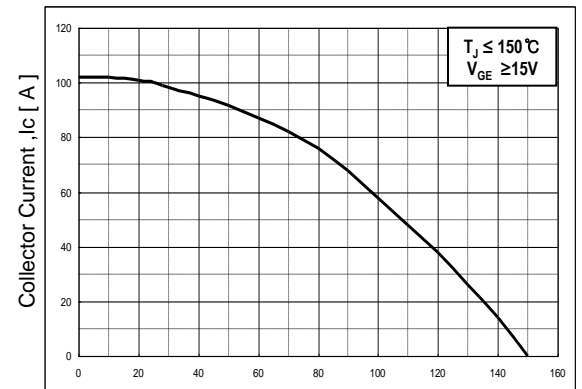
Fig 12. rated Current vs. Case Temperature
