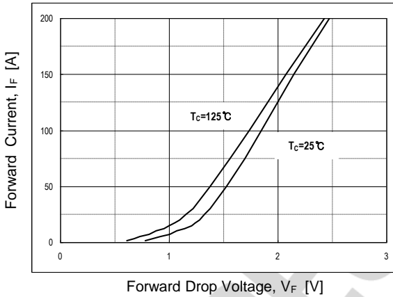
Fig 15. Forward characteristics
