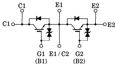
EQUIVALENT CIRCUIT
