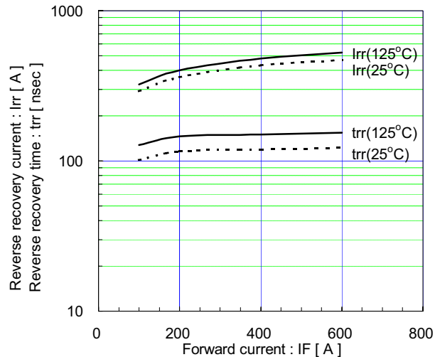
Reverse recovery characteristics (typ.) Vcc=600V, VGE=±15V, RG=1.5Ω
