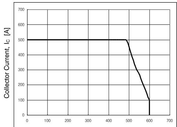
Collector-Emitter Voltage, V_{CE} [V]
