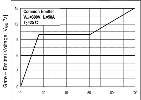
Gate Charge, Q_g [nC]
