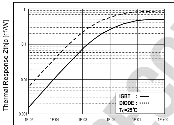
Rectangular Pulse Duration Time [sec]
