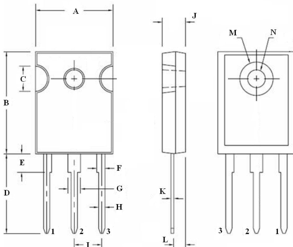
APQ65SN06AD-XXM0 TO-247
