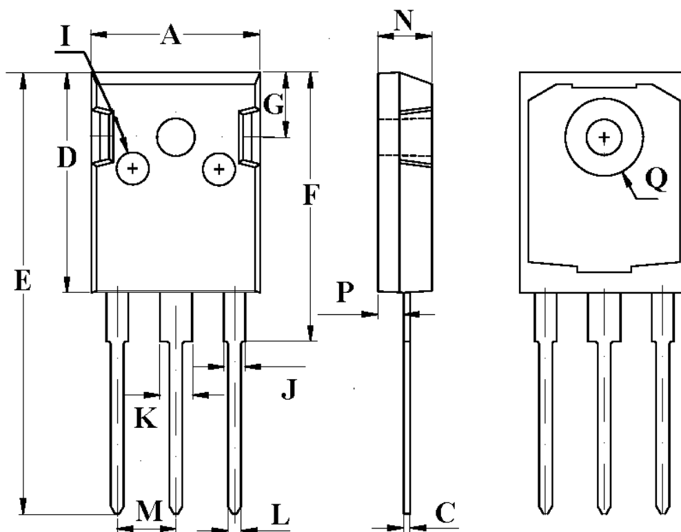
APQ65SN06AD-XXJ0 TO-247
