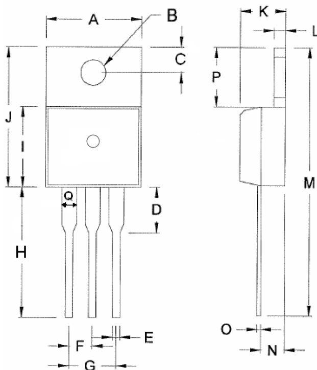
APQ65SN06AH—XXM0 TO-220
