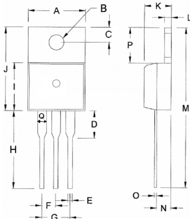
APQ50SN06AH-XXM0 TO-220
