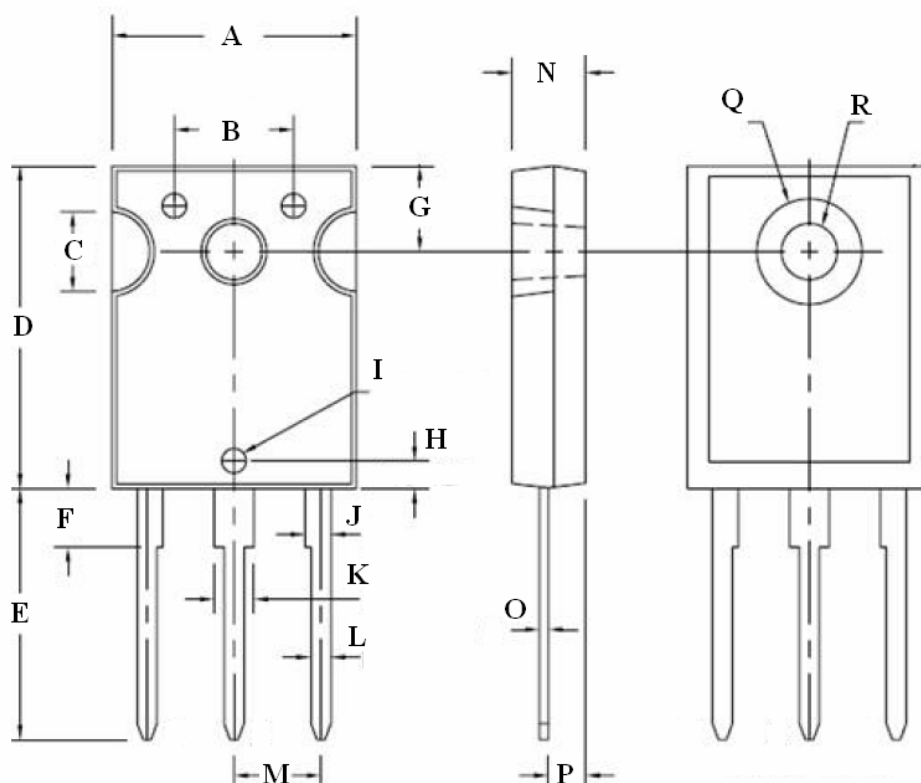
APQ09SN90AD-XXM0 TO-247
