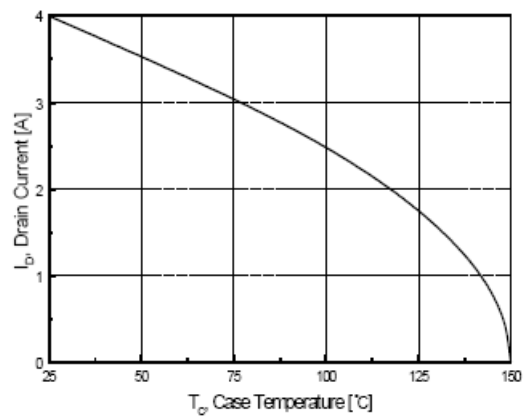
Fig. 6 Maximum Drain Current vs Case Temp.
