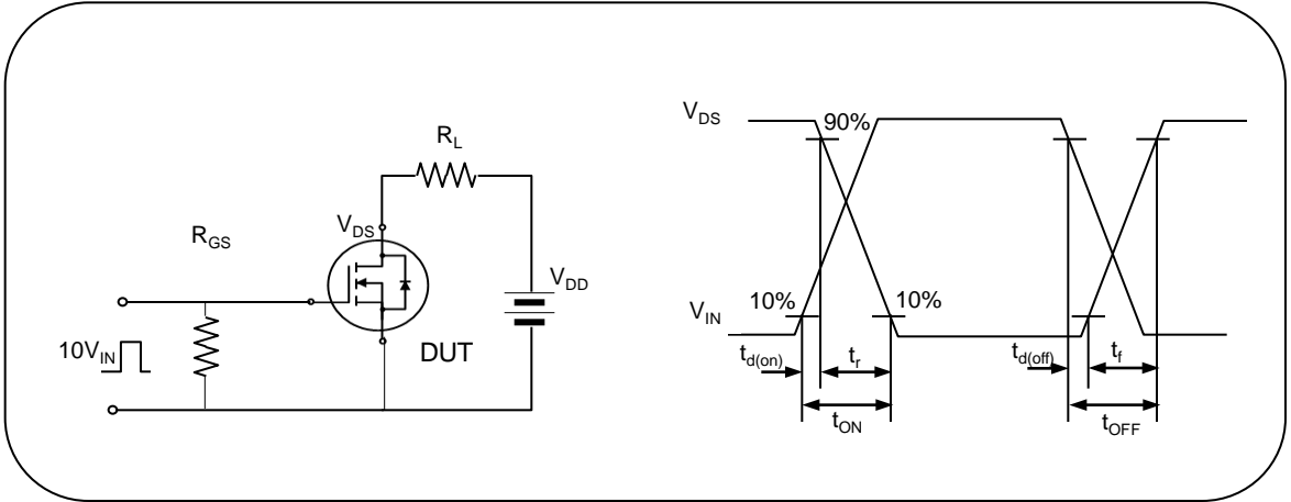
Fig. 12. Switching time test circuit & waveform
