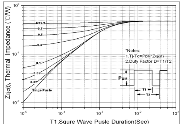
Fig. 10. Transient thermal response curve (TO-251)
