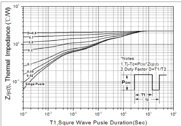
Fig. 9. Transient thermal response curve (TO-220F)
