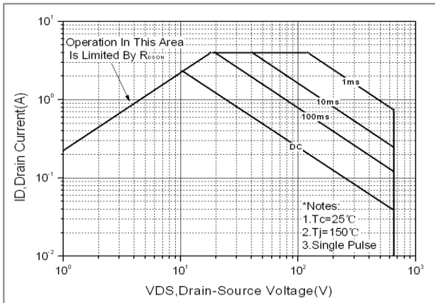
Fig. 9. Maximum safe operating area (TO-251N&TO-251S)
