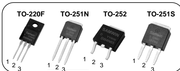
1. Gate 2. Drain 3. Source
