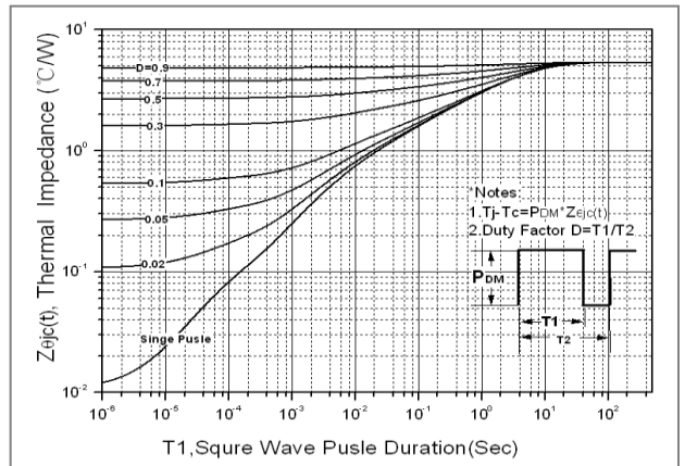
Fig. 10. Transient thermal response curve (TO-251N&TO-251S)
