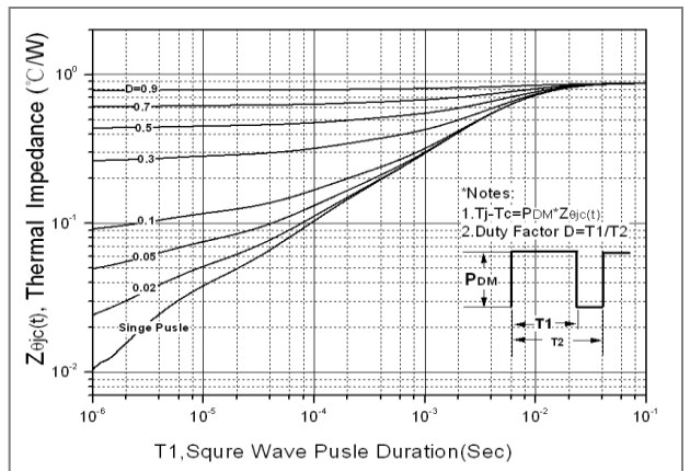
Fig. 12. Transient thermal response curve (TO-252)
