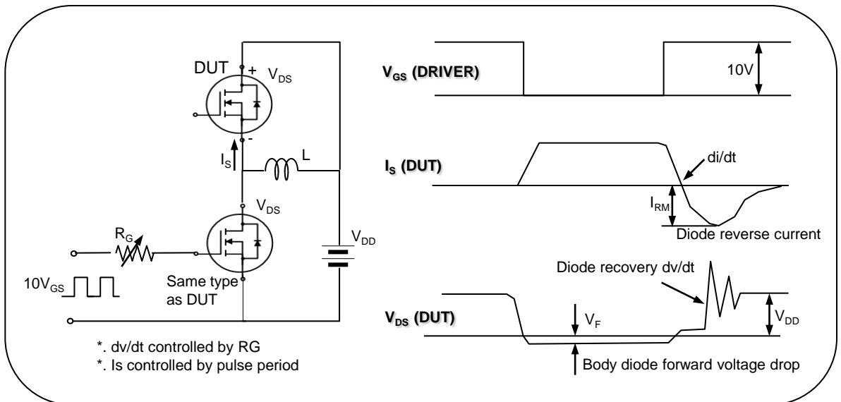
Fig. 17. Peak diode recovery dv/dt test circuit & waveform
