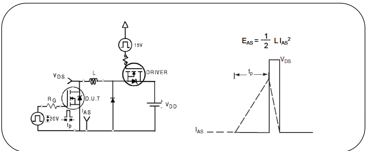
Fig. 14. Unclamped Inductive switching test circuit & waveform
