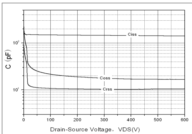
Fig. 11. Capacitance Characteristics
