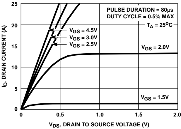
FIGURE 7. SATURATION CHARACTERISTICS
