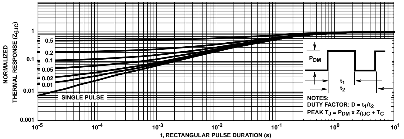
FIGURE 7. NORMALIZED MAXIMUM TRANSIENT THERMAL RESPONSE
