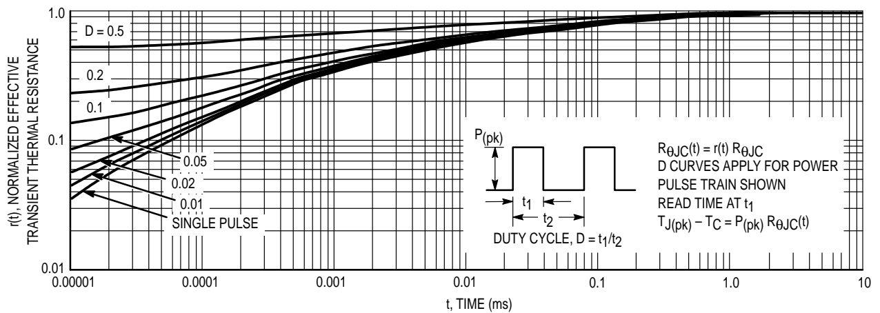
Figure 13. Thermal Response
