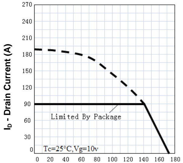
Drain Current
