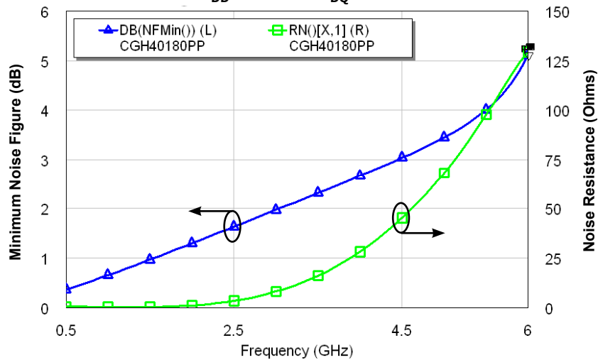
Simulated Minimum Noise Figure and Noise Resistance vs Frequency of the CGH40180PP V_{DD} = 28\text{ V}, I_{DQ} = 1\text{ A}
