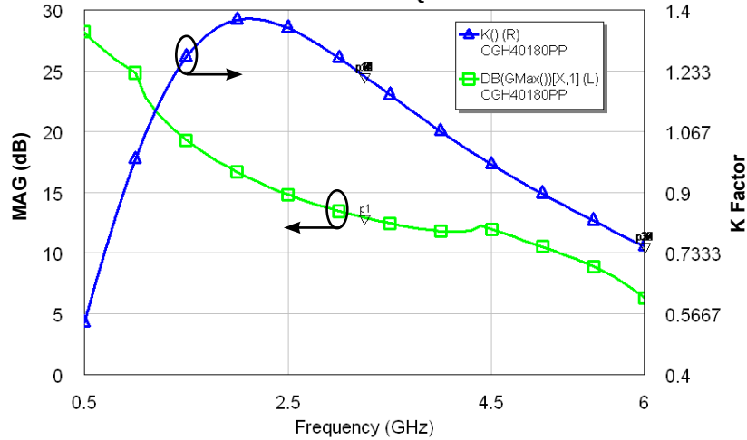
Simulated Maximum Available Gain and K Factor of the CGH40180PP V_{DD} = 28\text{ V}, I_{DQ} = 1.0\text{ A}
