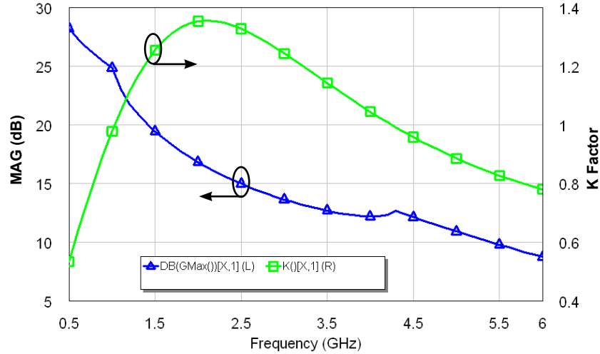
Simulated Maximum Available Gain and K Factor of the CGH40120 V_{DD} = 28\text{ V}, I_{DQ} = 1.0\text{ A}
