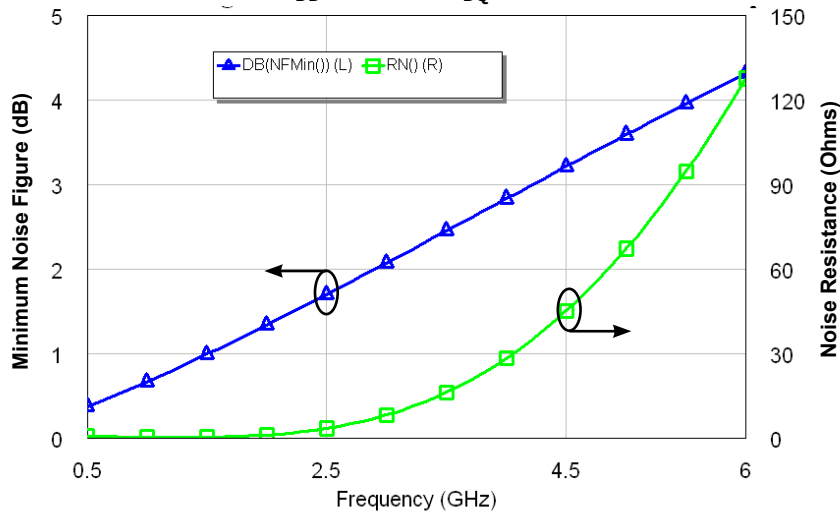
Simulated Minimum Noise Figure and Noise Resistance vs Frequency of the CGH40120 V_{DD} = 28\text{ V}, I_{DQ} = 1\text{ A}
