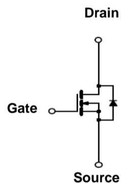
N-Channel MOSFET
