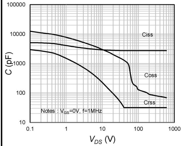
Fig.8 Capacitance Characteristics
