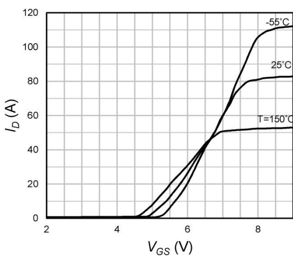
Fig.5 Transfer Characteristics
