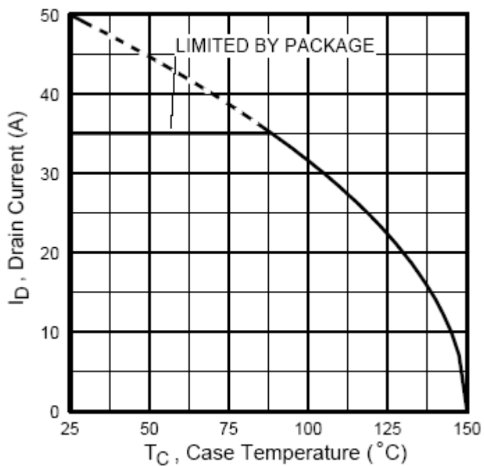
FIGURE 4. Maximum drain current vs case temperature - Continued.
