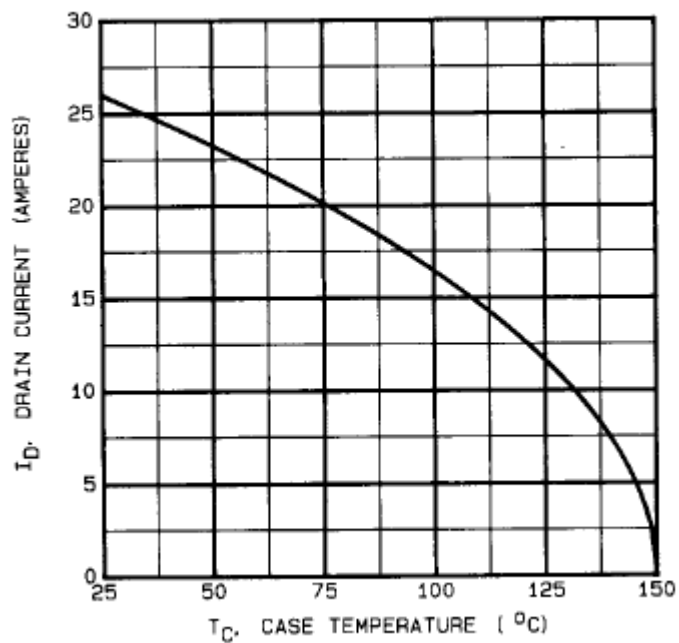
FIGURE 4. Maximum drain current vs case temperature.
