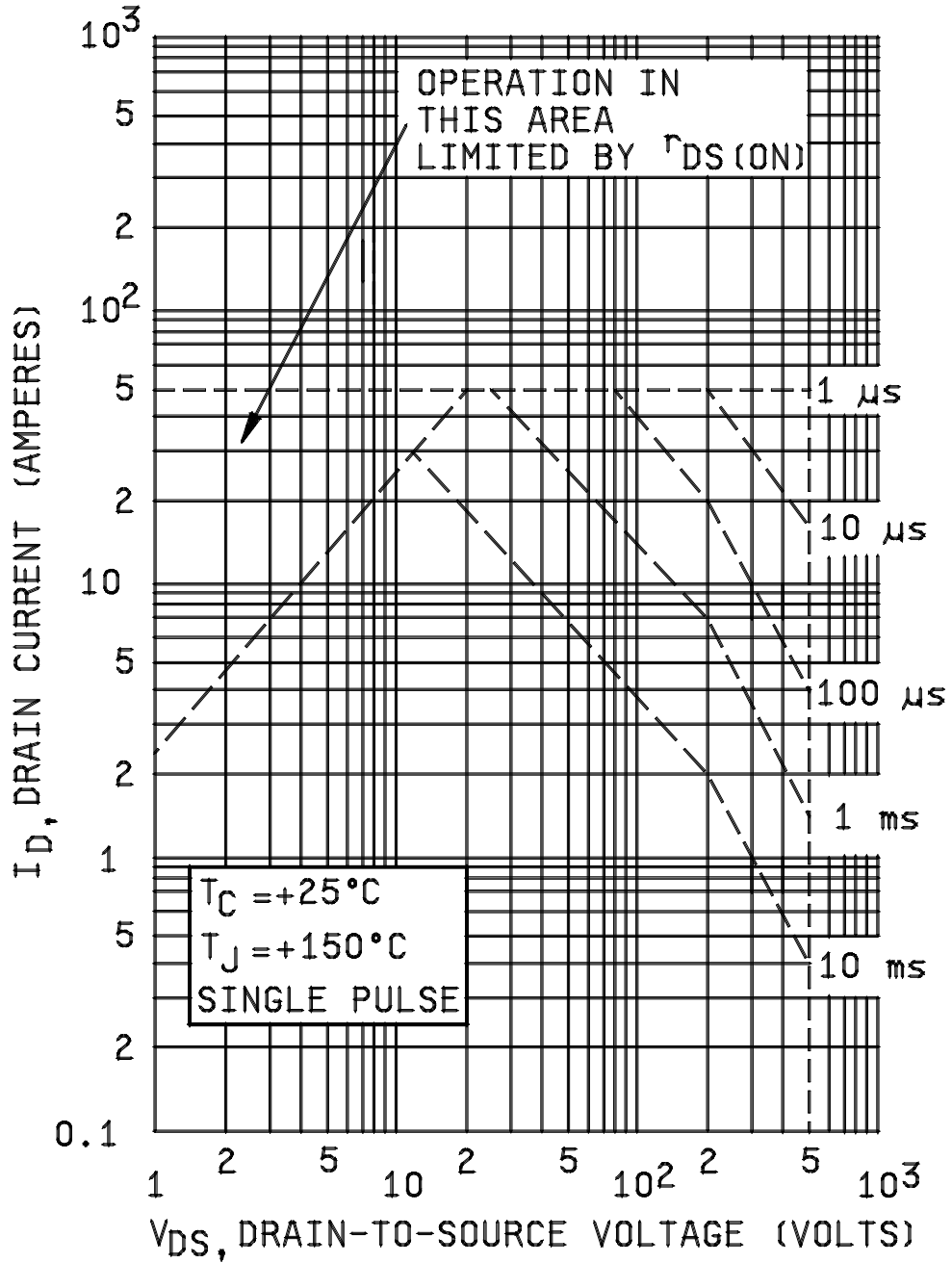
FIGURE 8. Safe operating area graph.
