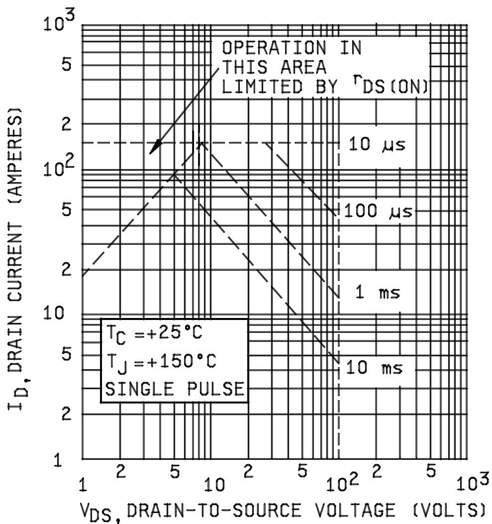
FIGURE 6. Safe operating area graph.
