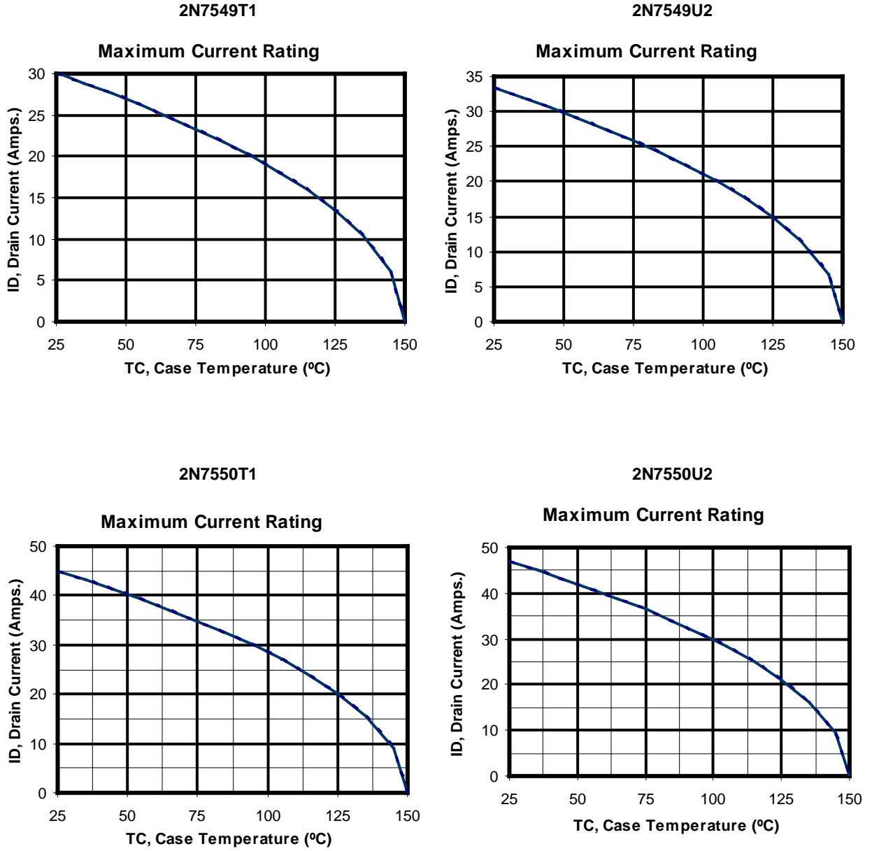
FIGURE 4. Maximum drain current versus case temperature graphs.
