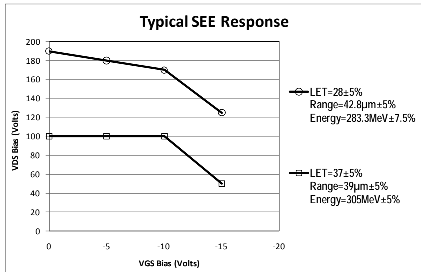
FIGURE 5. Typical single event effects safe operating area graphs.
