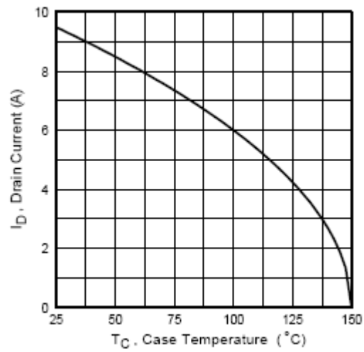
FIGURE 3. Maximum drain current versus case temperature graphs.
