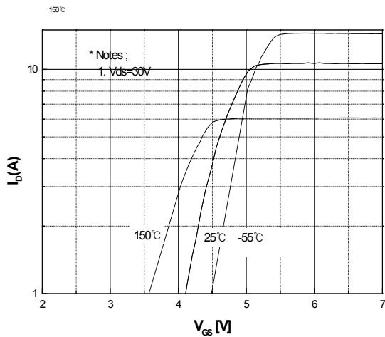
Fig.5 Transfer Characteristics
