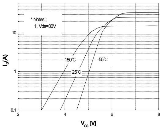
Fig.5 Transfer Characteristics
