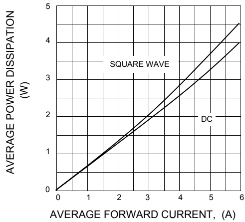
FIG.2 - POWER DISSIPATION
