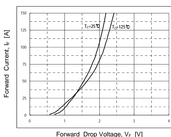
Fig 12. Forward characteristics
