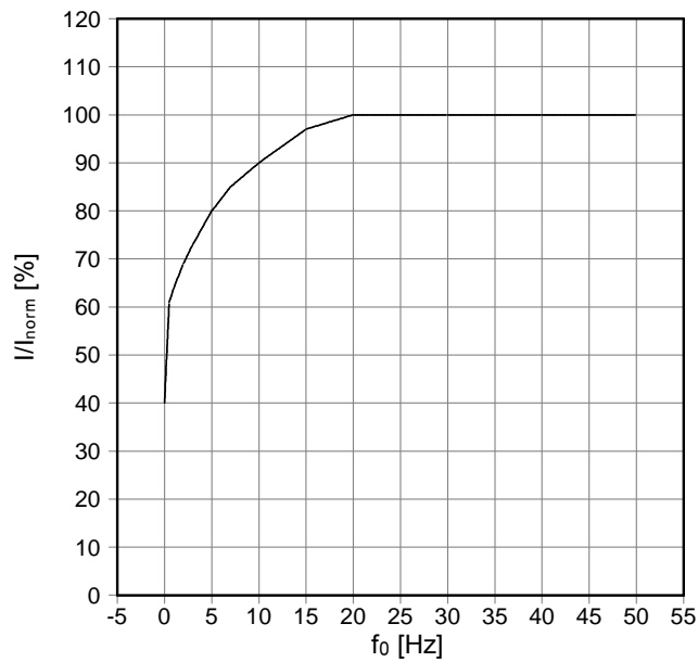
fo - derating curve IGBT (motor) cos(phi) = 0,95 T cool medium = 50°C
