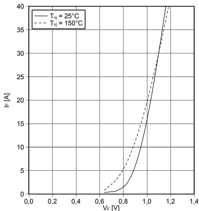
順方向特性 逆極性保護diodeB ( 典型 ) forward characteristic of Inverse-polarity protection diode B (typical) I_F = f(V_F)
