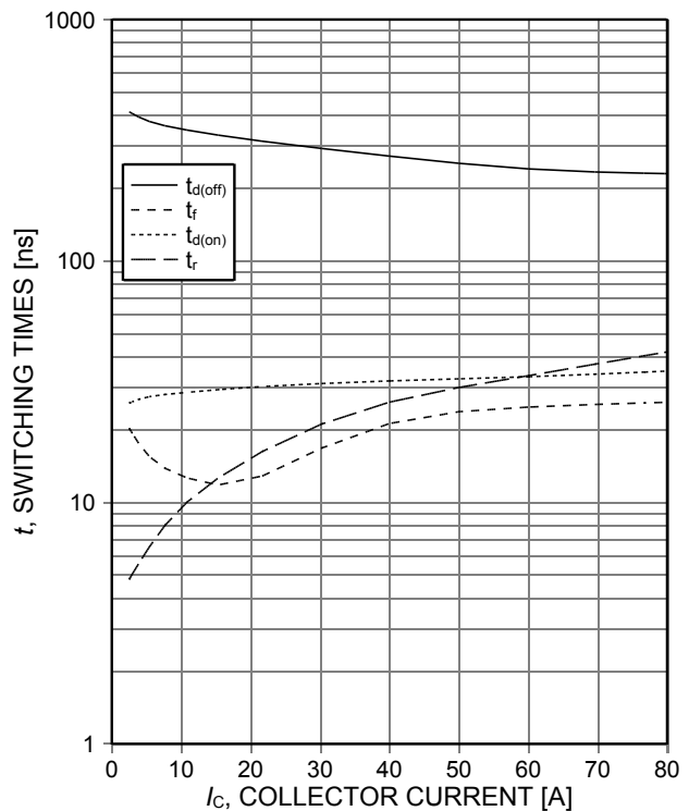
Figure 8. Typical switching times as a function of collector current (inductive load, T_j=175^\circ\text{C} , V_{CE}=400\text{V} , V_{GE}=15/0\text{V} , r_G=10\Omega , Dynamic test circuit in Figure E)
