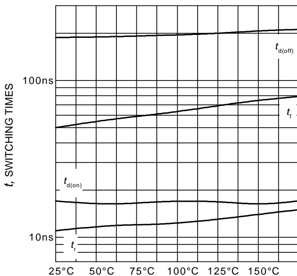
Figure 11. Typical switching times as a function of junction temperature (inductive load, V_{CE} = 400\text{V} , V_{GE} = 0/15\text{V} , I_C = 15\text{A} , r_G = 15\Omega , Dynamic test circuit in Figure E)
