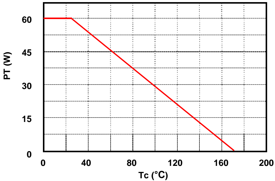
Power Dissipation vs. Case Temperature
