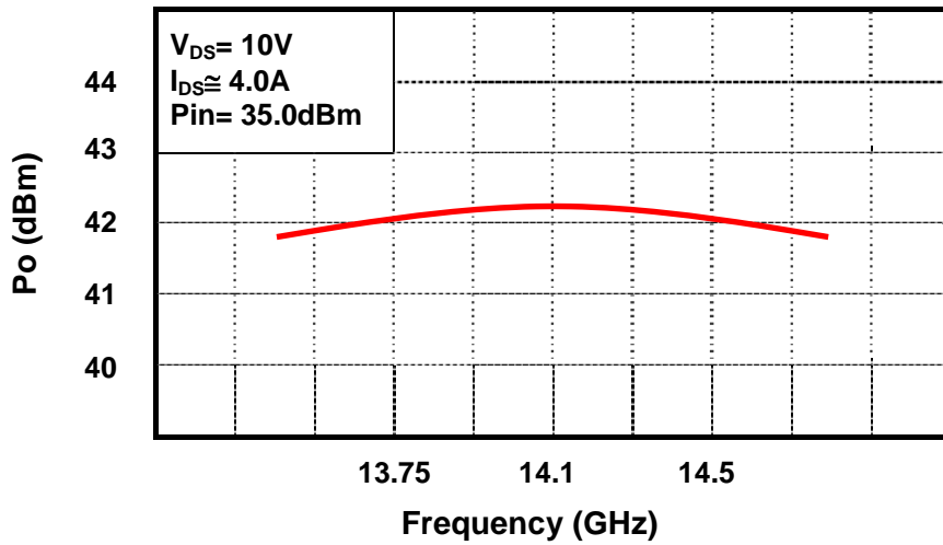
Output Power vs. Frequency
